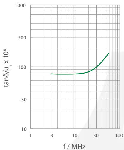
\tan\delta / \mu_i
