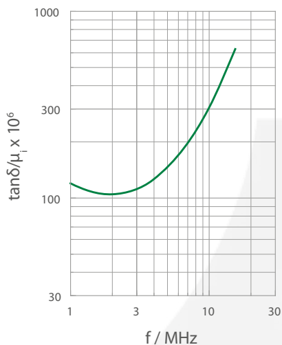
\tan\delta / \mu_i
